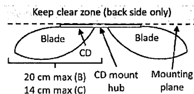
Example Assembly Side / Top View
